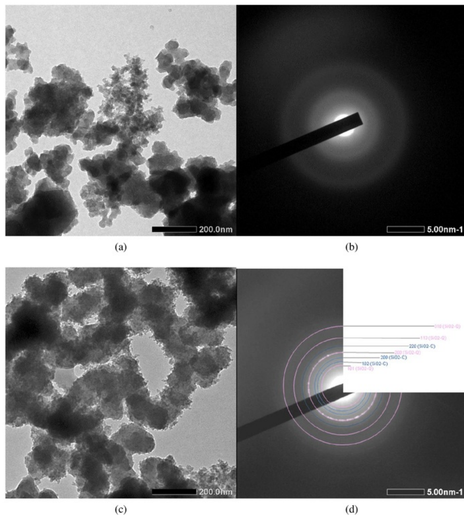
Fig. 6. TEM with electron diffraction images of \text{SiO}_2 nanoparticles: (a) and (b) – NS(3); and (c) and (d) – NS(6).
